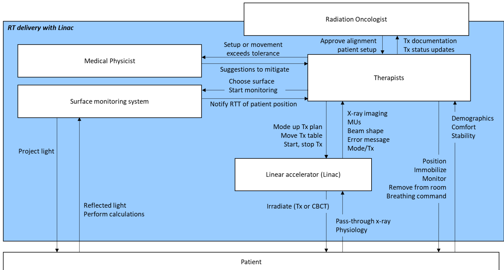
Figure 32 The part of the SCS showing the details of RT delivery (linac)
